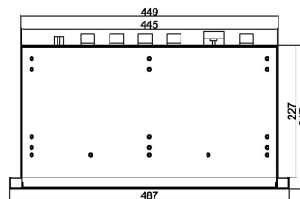
[평면도]
