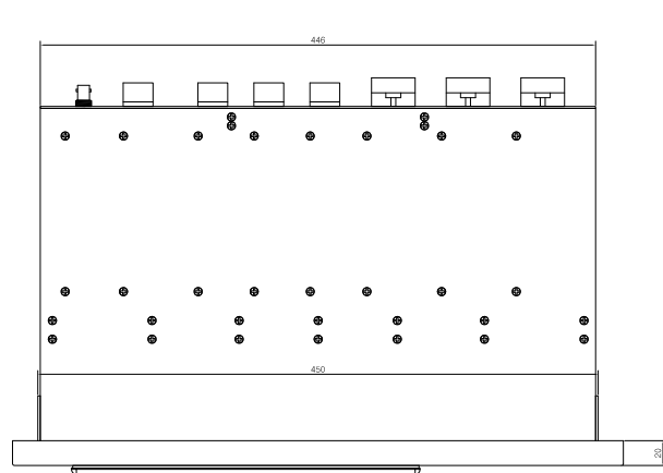
[평면도]
